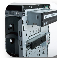
Removable drive bay cage easy but robust drive locking system
